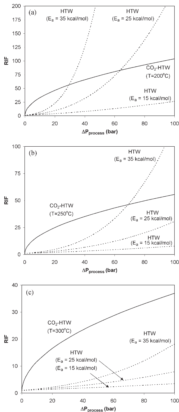
Figure 6. RIF as a function of \Delta P_{\text{process}} for \text{CO}_2 -enriched HTW at constant temperature ( \text{CO}_2\text{-HTW} ) and for increased-temperature HTW (HTW).
